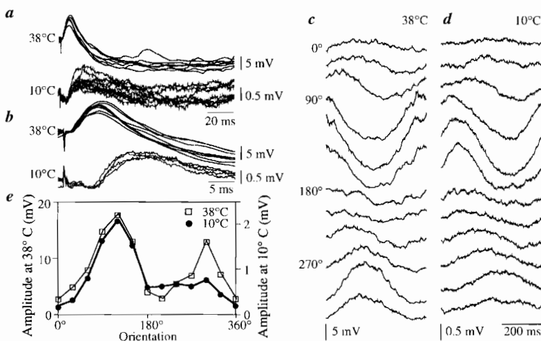
FIG. 3 The effects on the visually and electrically evoked responses of a second simple cell. The layout is identical to that of Fig. 1. Slight shifts in the temporal phase of some of the visually evoked responses were apparent during cooling (compare c and d ). These shifts were not present in the cell shown in Fig. 1. They were probably caused by small (<0.5°) shifts in the position of the eyes; in other cells, similar shifts over time were observed independently of cooling. In this cell, cooling increased direction selectivity.
