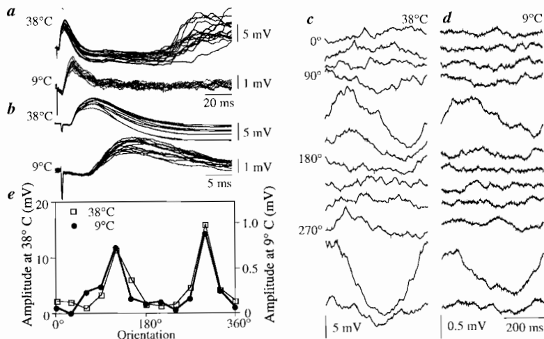
FIG. 1 The effects of cooling on the visually and electrically evoked responses of a layer-4 simple cell. a , response of a simple cell to electrical stimulation of the LGN (1 mA, 200 \mu s) recorded at normal temperature and during cooling. b , Similar traces shown at a different time scale. The short (1.8 ms) and stable latency of the e.p.s.p. indicates that this cell received monosynaptic excitation from the LGN. The monosynaptic e.p.s.p. was followed by a long-lasting (150 ms) i.p.s.p. of disynaptic origin. When the cooling plate temperature was lowered to 9°C, the latency of the e.p.s.p. increased to 5 ms, its rise time was dramatically slowed, and its amplitude was reduced; the i.p.s.p. disappeared. c , The cell's response to drifting gratings of 12 different orientations. Each trace is the averaged response to 20 grating cycles. d , Responses to the same visual stimuli as in c , but with the cortex cooled. The responses are similar in shape to those in c , but more than 17-fold smaller in amplitude (note different vertical scales in the figure). e , Orientation tuning curves constructed from the records of c and d . Each point indicates the peak-to-peak amplitude of the first harmonic (2 Hz) component of the corresponding trace. Once again, note the different vertical scales for the two plots.
